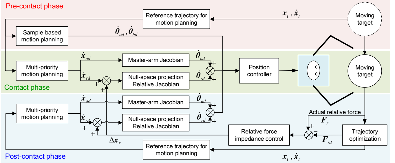
Fig. 2: Overview of the control pipeline for the capturing process. The whole process is decomposed into three phases: pre-contact phase (Section II), contact phase (Section III) and post-contact (Section IV). Note that the trajectory optimization is computed offline.
