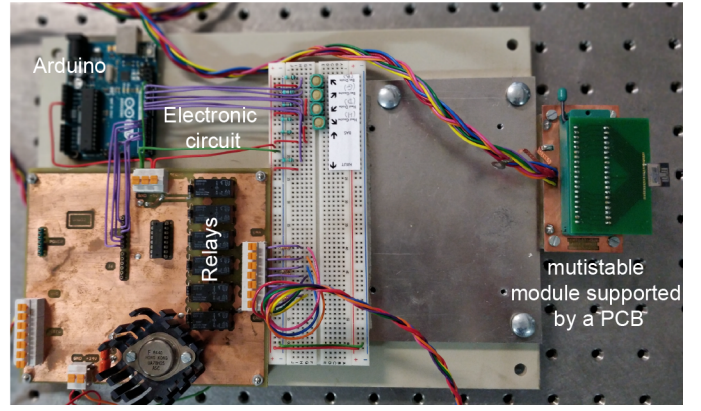
Fig. 8. Experimental Bench.
