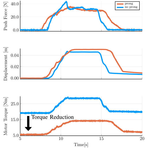
Fig. 6: Comparison of torso displacement, maximum push force and required motor torque (left front knee) when pushing the robot with (red) and without (blue) prongs.
