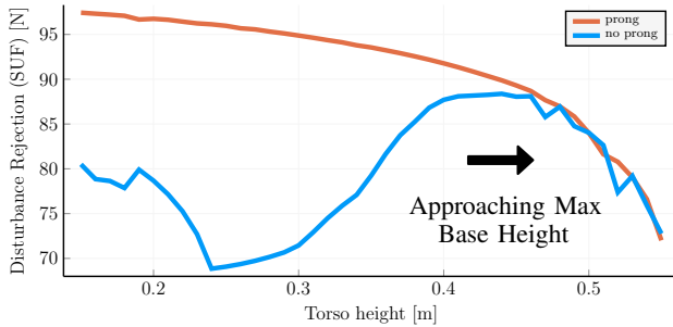
Fig. 3: The SUF for each height of the base. The foot locations are optimized for each height.
