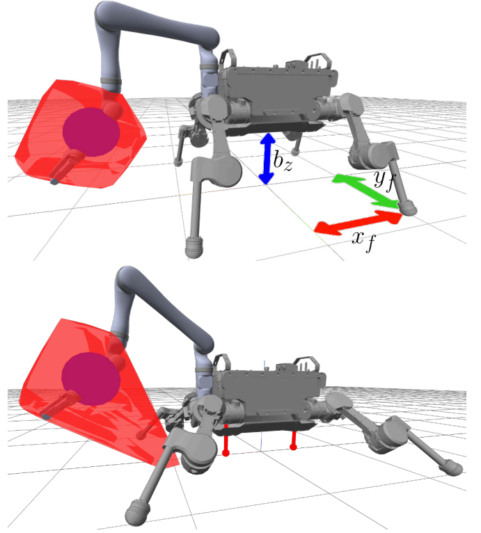
Fig. 2: Rejectable Force Polytope and maximal rejectable force for optimised robot configuration with prong (bottom) and without prongs(top). The end-effector is set to a world frame position: \{0.8\text{m}, 0.2\text{m}, 0.4\text{m}\} .
