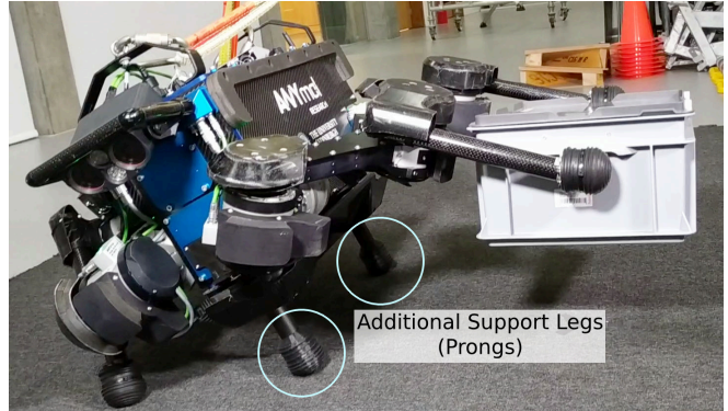
Fig. 1: Body-ground contact for enabling diverse loco-manipulation tasks: manoeuvring objects by legs.
