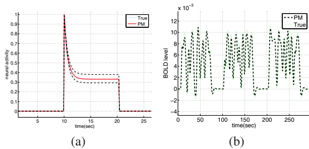
Fig. 1. (a): One pulse of the reconstructed and true neural activity. The shape of the signal is retrieved, although the slope is slightly off, corresponding to a bias in the \tau_i estimate. (b): Reconstructed and true BOLD signal (first 3 epochs).
