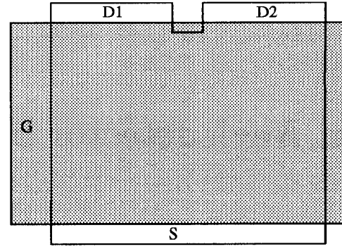
Figure 3. MAGFET Layout
