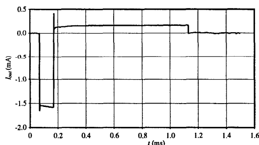
Figure 9. Measured output current pulse from the stimulator
