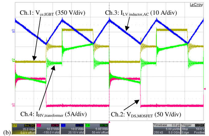
Fig. 2. Developed prototype of the dc-dc converter (a) and switching waveforms (b) at 60 V 40 A on the low voltage side and 750 V on the high voltage side in SOFC mode. Ch.1(yellow): V_{ce,IGBT} (350 V/div), Ch.2(red): V_{ds,MOSFET} (50 V/div), Ch.3(blue): I_{LV,inductor,AC} (10 A/div), Ch.4(green): I_{HV,transformer} (5 A/div). Time 5μs/div.
