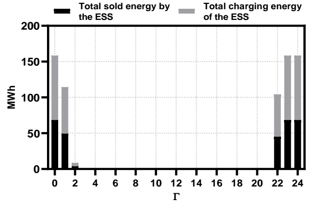
Fig. 8. Total purchased and sold energy by the ESS in the entire scheduling horizon for different values of \Gamma .
