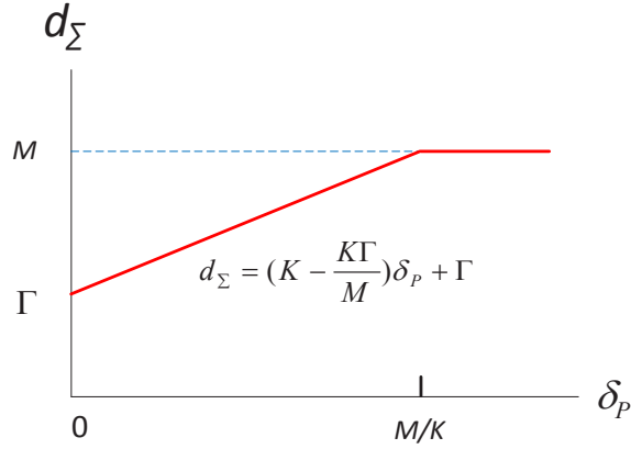
Fig. 5. Achievable sum DoF d_\Sigma vs. \delta_P for the MISO BC with M < K .
