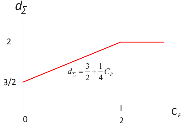
Fig. 3. Optimal sum DoF ( d_\Sigma ) vs. total perfect CSIT feedback cost ( C_P ) for three-user 2 \times 1 MISO BC.
