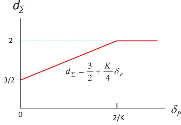
Fig. 4. Achievable sum DoF d_\Sigma vs. \delta_P for the K(\geq 3) -user 2 \times 1 MISO BC.
