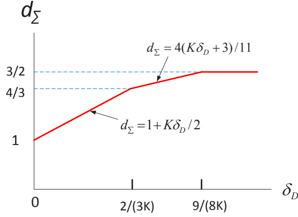
Fig. 6. Achievable sum DoF d_\Sigma vs. \delta_D for the MISO BC with K \geq 3, M = 2 , where \delta_P = 0 .
