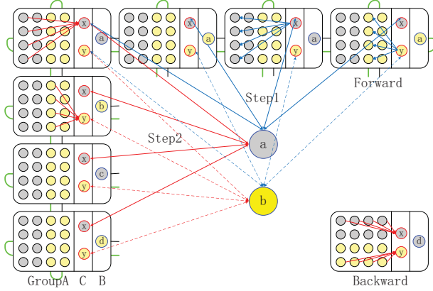
(a) Mapping on SpiNNaker using pipelined model (PCBP).
