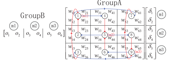
(a) Checkerboarding partitioning.
