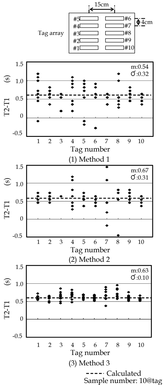
Fig. 8. Different time between two antennas
