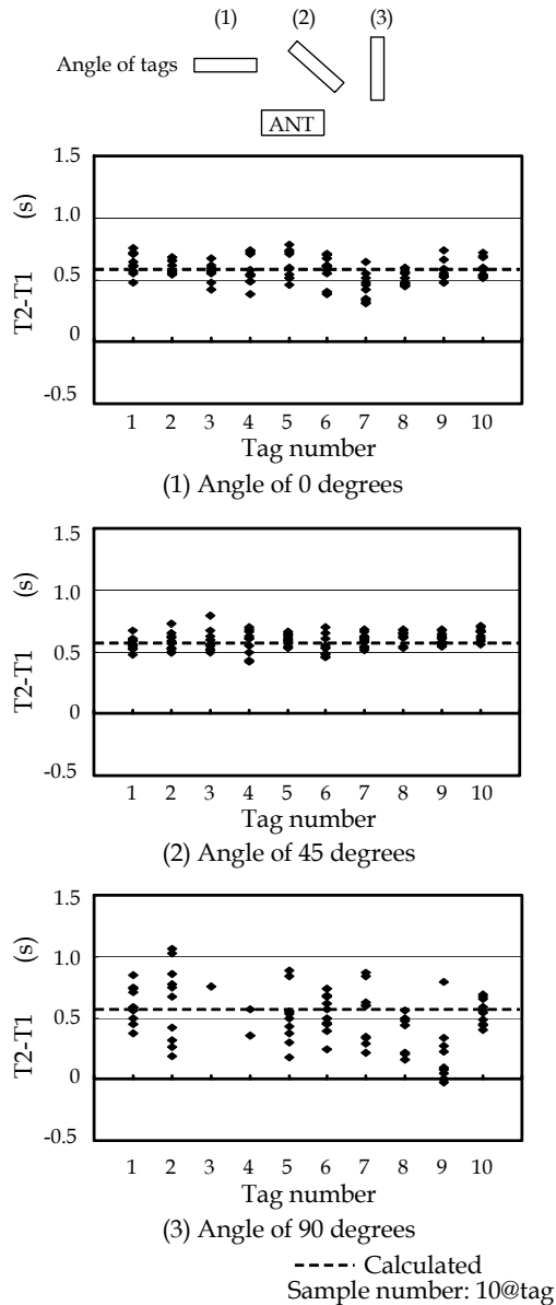
Fig. 14. Different time between two antennas
