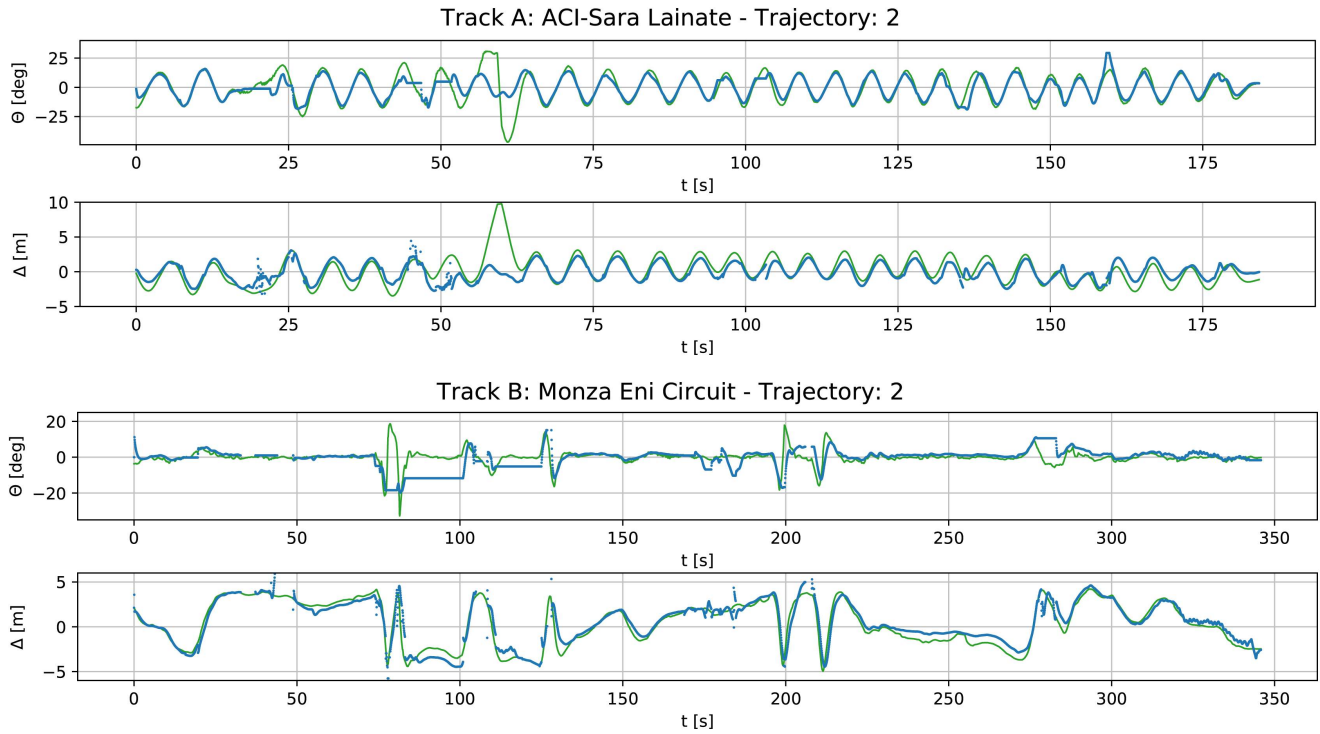
Fig. 8. Examples of the experimental results obtained in oscillating and racing driving styles, designed to stress the estimation of, respectively, heading (top) and lateral displacement (bottom). The graphs compare the estimates (in blue) with the respective ground truth (in green).
