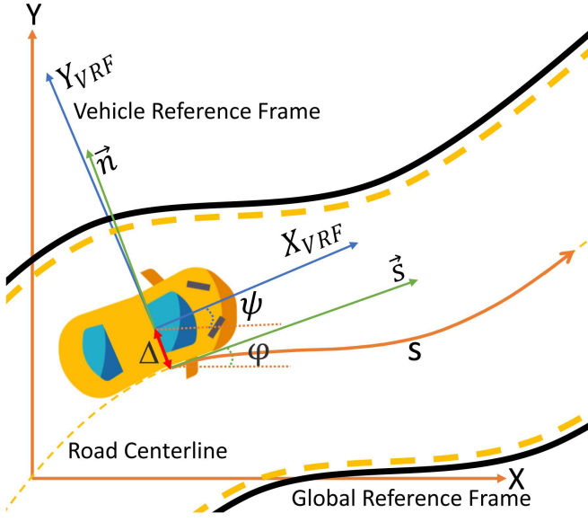
Fig. 2. Road representation used in lateral control, highlighting the road centerline as a parametric curve in the vehicle reference frame, and the vehicle relative pose as heading \Theta = \varphi - \psi and lateral displacement \Delta .
