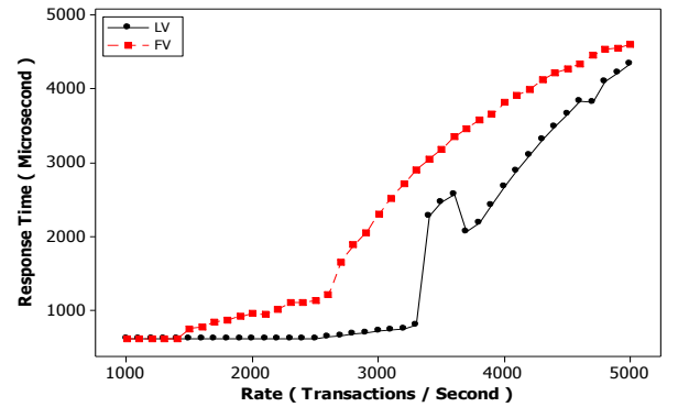
Fig. 4: Average response time with 75 % update transactions
