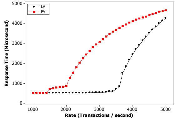
Fig. 3: Average response time with 50 % update transactions
