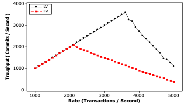
Fig. 1: Throughput with 50 % update transactions
