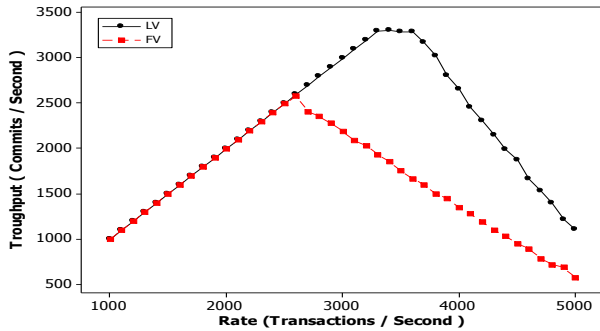
Fig. 2: Throughput with 75 % update transactions
