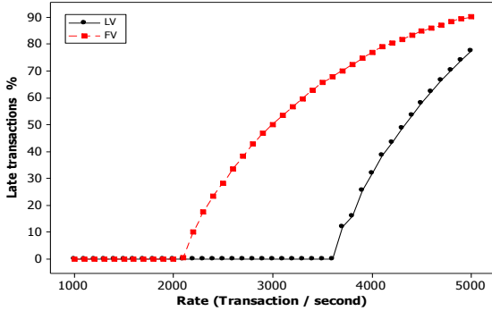
Fig. 5. Late transactions with 50 % update transactions
