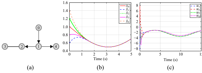
Fig. 1. The communication topology and trajectories of \hat{x}_i , x_0 , and u_i . (a) The interactions among the agents; (b) The responses of \hat{x}_i and x_0 ; (c) Evolutions of control inputs u_i .
