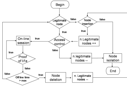
Figure 1: Node Life-Cycle
