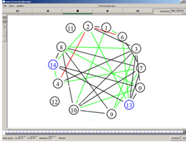
Figure 2: Example of Final Associated Graph and Hamiltonian Cycle
