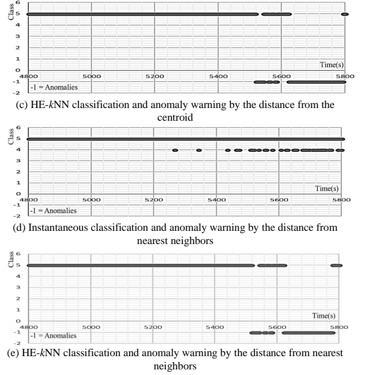
Fig. 9. Waveforms and results from the ELV dc air conditioner on malfunction in fan
