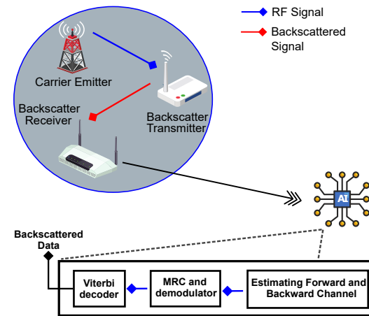
Fig. 5: Illustration of AI-based Solutions for Backscatter Signal Detection and Channel Estimation
