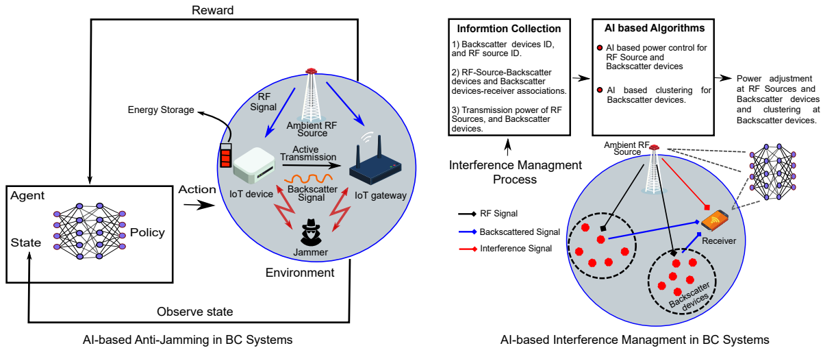
Fig. 6: Illustration of AI-based jamming/security and interference management in BC networks.
