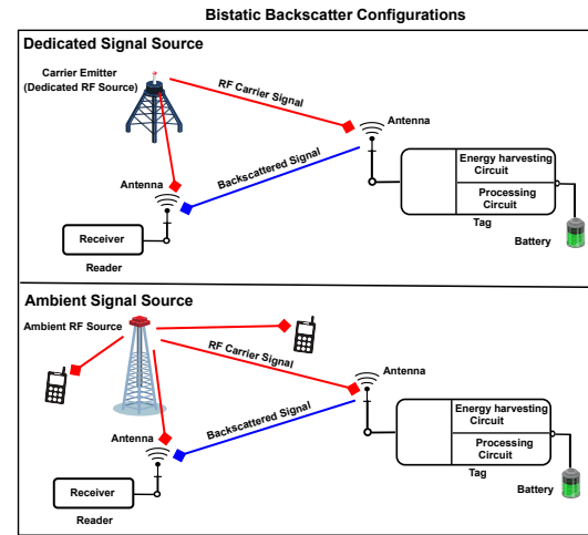
Fig. 2: Illustration of bistatic configuration with a dedicated and ambient signal source.
