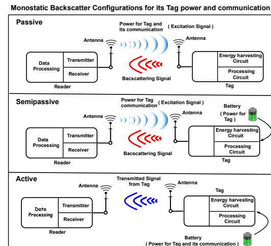
Fig. 3: Illustration of monostatic configurations that include passive, semi-passive, and active.
