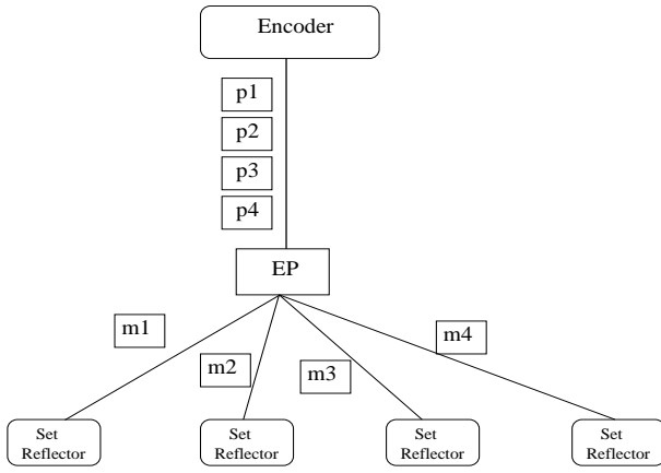
Fig. 7. Multipath error correction scheme.
