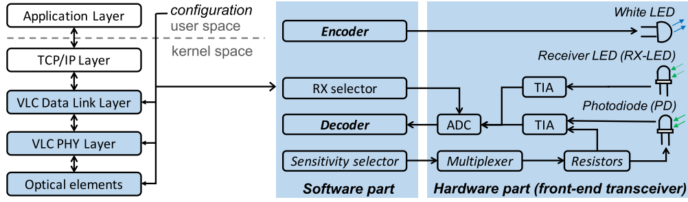
Fig. 12. System architecture: left ) communication stack; right ) block diagram of the front-end transceiver.
