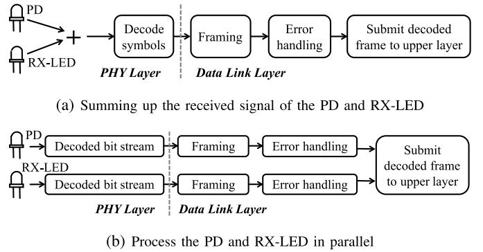
Fig. 14. Process the received signals from the PD and RX-LED at the receiver.
