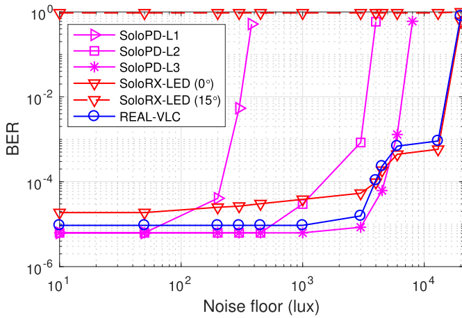
Fig. 16. The BER performance under different light conditions. In this figure, ‘SoloRX-LED (0°)’ denotes the scenario where the RX-LED and the transmitter are well aligned. Similarly, ‘SoloRX-LED (15°)’ denotes the scenario that the RX-LED and the transmitter are misaligned by an angle of 15° (the FOV of the RX-LED is 8°). The BER under REAL-VLC increases significantly to nearly 100% when the noise floor reaches 2 \times 10^4 because the RX-LED has been saturated.
