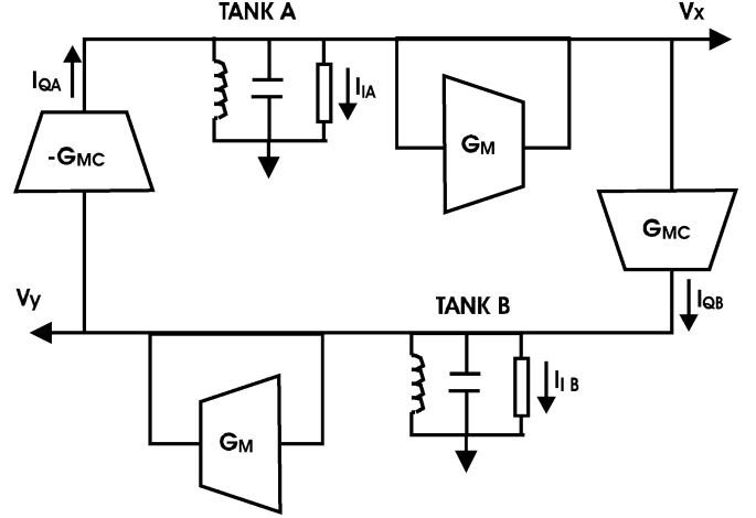
Fig. 2. Simplified linear model for a QVCO.
