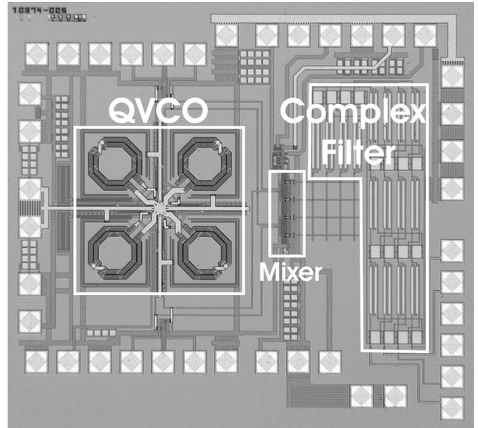
Fig. 8. Chip photograph of the new TS-QVCO, together with the SSB upconversion circuits (1.5 mm \times 1.8 mm).
