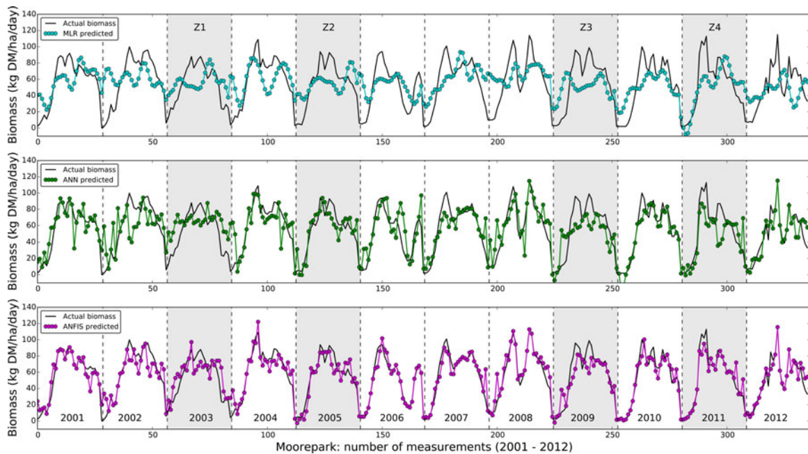
Fig. 10. Plots of observed and modeled time series by using MLR, ANN and ANFIS for Moorepark study site. The shaded regions Z1 (2003), Z2 (2005), Z3 (2009) and Z4 (2011) were selected for more detailed analysis (see Fig. 11).
