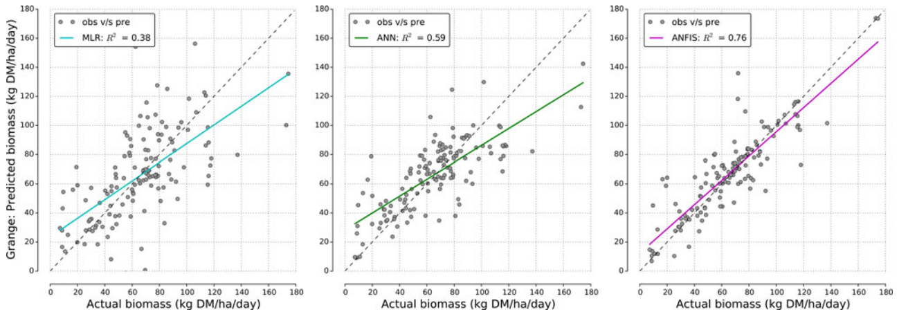
Fig. 12. Scatter plots for the accuracy comparison of MLR, ANN and ANFIS estimated grassland biomass verses in situ biomass for Grange test site.
