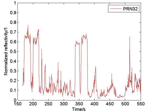
Fig. 7. Normalized power reflectivity of PRN32.
