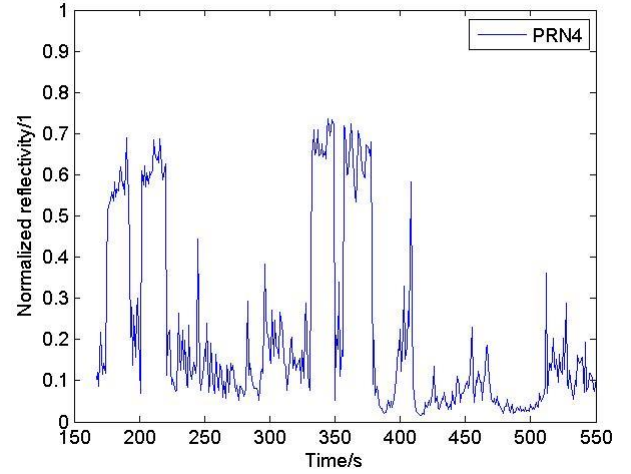
Fig. 6. Normalized power reflectivity of PRN4.
