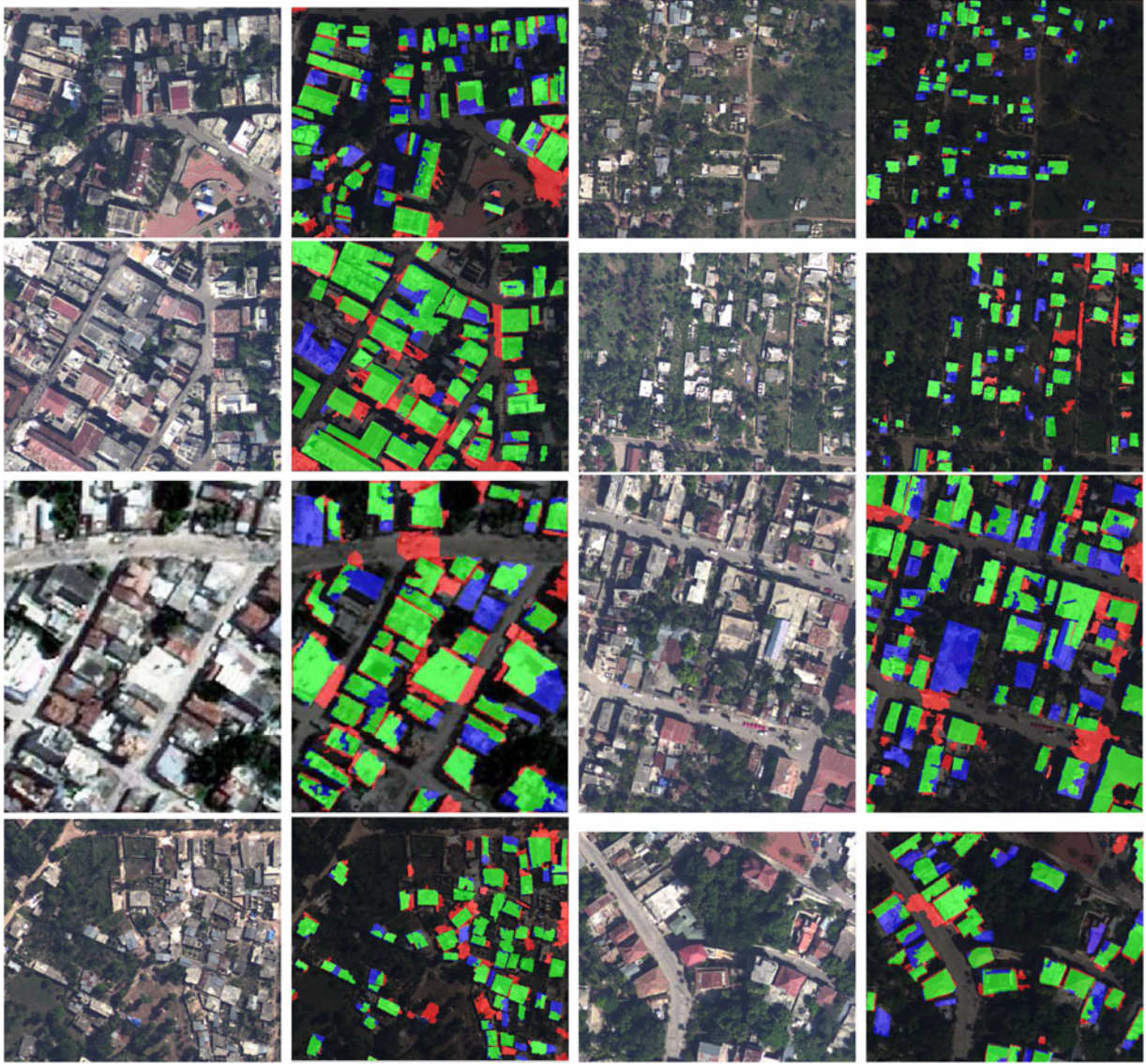
Fig. 8. The results of the proposed approach on NOAA images: (First column) Test images #1–4. (Second column) Detected buildings for test images #1–4. (Third column) Test images #5–8. (Fourth column) Detected buildings for test images #5–8.
