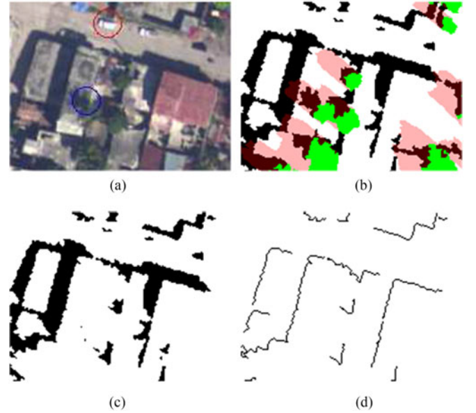
Fig. 3. Building Shadow boundary detection. (a) RGB image. Shadow is cast by vegetation (blue circle) or other small nonbuilding objects such as vehicle (red circle). (b) Shadow M_S (black) and vegetation M_V (green). The expansion regions (pink color) are generated by dilating vegetation objects. (c) Shadow mask after eliminating shadows generated by vegetation. (d) Building shadow boundary mask M_{SB} .
