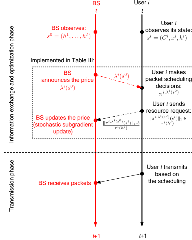
Fig. 3. Illustration of the interaction between the BS and user i (i.e. their decision making and information exchange) in one period.
