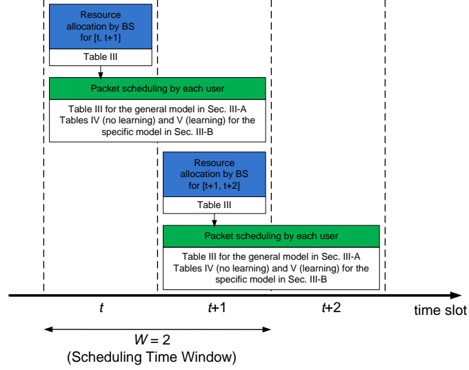
Fig. 2. Illustration of the resource allocation and packet scheduling in the proposed solution.
