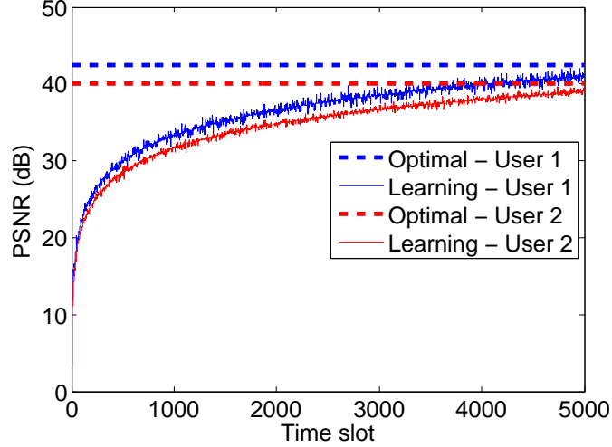
Fig. 4. Convergence of the PDS-based learning algorithm.
