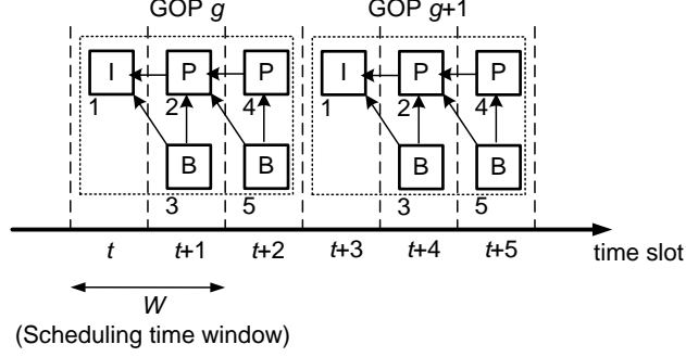
Fig. 1. Illustration of GOP (group of pictures), DU (data unit), and packet scheduling. Since the scheduling time window is W = 2 , the contexts in different time slots are C_t = \{DU_1^g, DU_2^g, DU_3^g\} , C_{t+1} = \{DU_2^g, DU_3^g, DU_4^g, DU_5^g\} , C_{t+2} = \{DU_4^g, DU_5^g, DU_1^{g+1}\} , C_{t+3} = \{DU_1^{g+1}, DU_2^{g+1}, DU_3^{g+1}\} , and so on.
