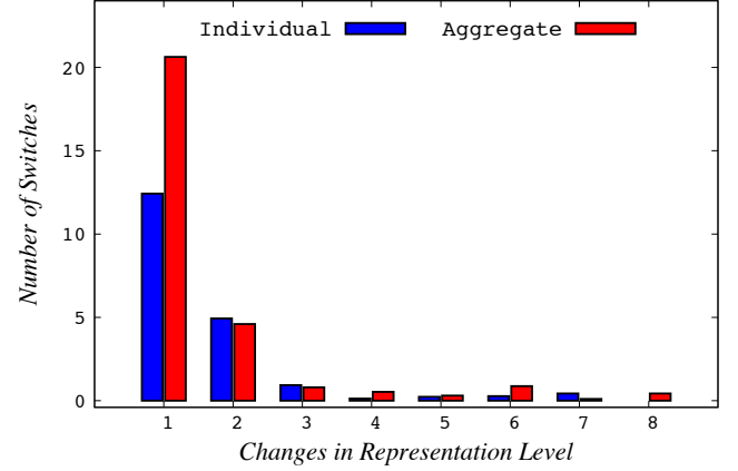
Figure 5: Switching dynamics - representation variations encountered in the Individual and Aggregated cases
