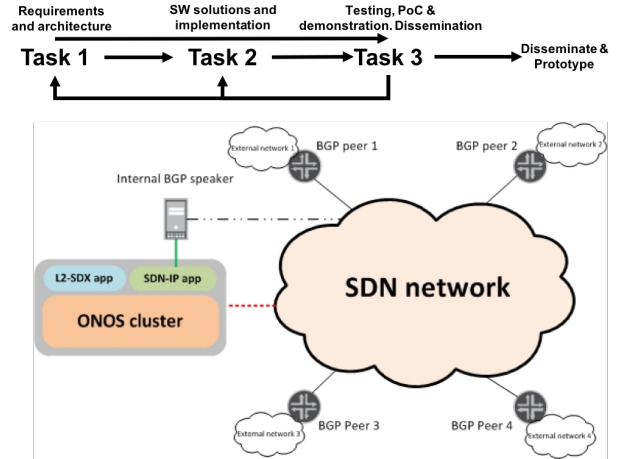
Fig. 1: Development process and SDN based OXP architecture these, are the Intents , which provide applications with a simple and powerful abstraction of end-to-end network connectivity. Using Intents, developers can rely on high-level network services abstractions. GÉANT Open service is composed by an existing ONOS application (SDN-IP [6]) and by a new ONOS application called L2-SDX. Both are available under Apache 2.0 Open Source license. SDN-IP is shipped within ONOS, L2-SDX can be downloaded from [7]. The Intent framework has been widely used for developing the SDN-IP and L2-SDX services.
