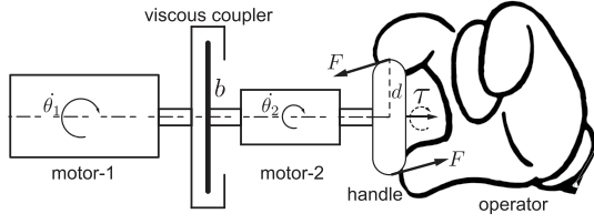
Fig. 4. Dual-stage haptic feedback device. The output torque is provided by the velocity of the large motor, through a viscous coupler, and the small one compensates the following error.
