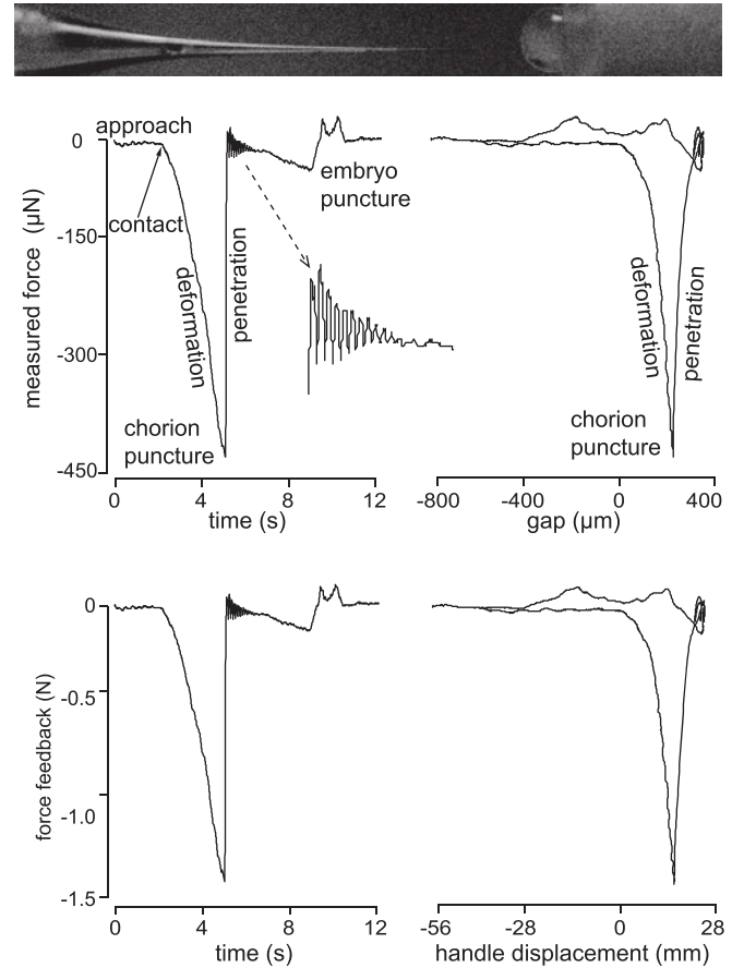
Fig. 9. Injection of dye in a zebra fish embryo. As on the trout egg experiment, the systems exhibited a very high transparency between micro and macro-scales.
