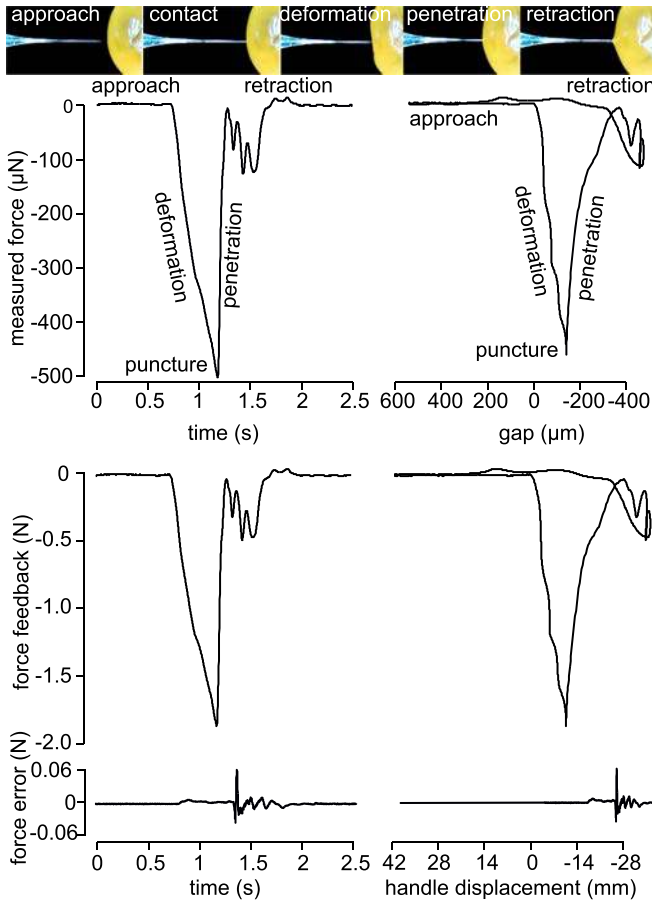
Fig. 8. Interaction with a hard trout egg. The force reflected to the user (central curve) was near-perfect linear amplification of the measured interaction (top curve).
