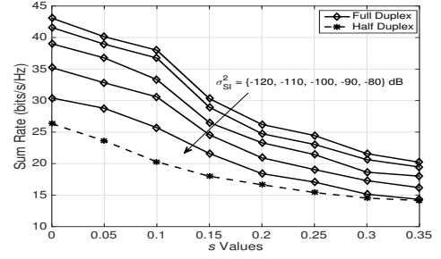
Fig. 1. Comparison between FD and HD systems with respect to s .
