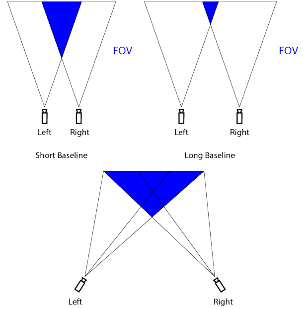
Fig. 3. Stereo vision system baseline and orientation
