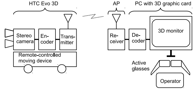
Fig. 1. Block diagram of the 3D video communication system for real-time remote control.
