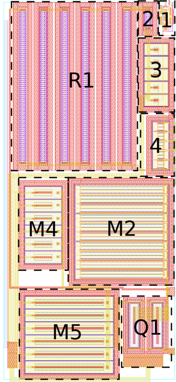
Fig. 5. Layout of the design in high-voltage 0.18 \mu\text{m} technology.
