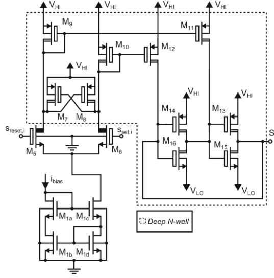
Fig. 1. Pulse-triggered level shifter extracted from [1].
