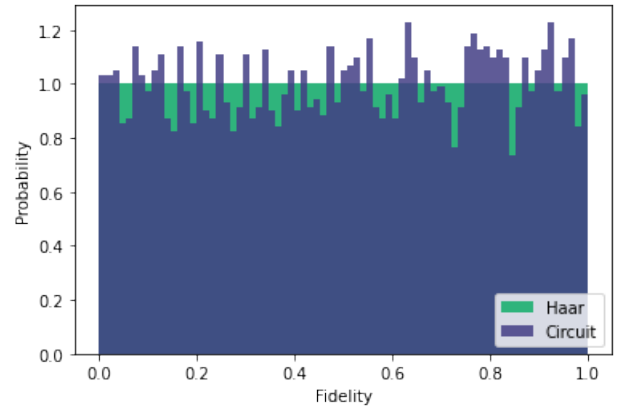
Fig. 4. Fidelity distribution of PQC overlaid on Haar fidelity distribution using non-uniform sampling
