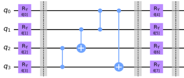
Fig. 11. Circuit 6
