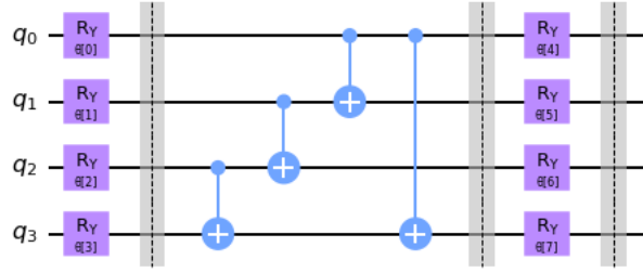
Fig. 6. Circuit 1
