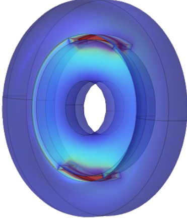
Fig. 6: Three-dimensional superconducting RF (SRF) cavity and electro-optic design for quantum transduction.
