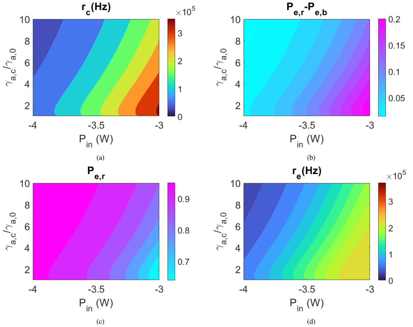
Fig. 7: Detector click rate r_c (a), difference between entanglement generation probability with red- and blue- detuning case P_{e,r} - P_{e,b} (b) entanglement generation probability in red-detuning case P_{e,r} (c) and entanglement rate r_e (d) as a function of the coupling strength \frac{\gamma_{a,c}}{\gamma_{a,0}} and input pump power P_{in} . It is important to emphasize that in some previous works [8] r_c expressed with (6) and P_{e,r} expressed with (13) are called entanglement rate and fidelity , respectively. However, in this case, r_e refers to the possibility of a single click of the detector and P_{e,r} refers to the probability that a single click of the detector indicates the presence of entanglement between distant processors.
