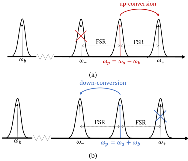
Fig. 2: Frequency spectrum for the output signal with red-detuned input pump power (a) and blue-detuned input pump power (b).
