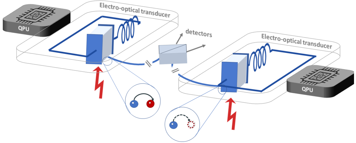
Fig. 5: M-M entanglement generation and distribution with red-detuned pump. Firstly, both microwave cavities are prepared with one photon state while leaving the optical cavity at the zero-photon state. A microwave photon can be converted to an optical photon (red circle).
