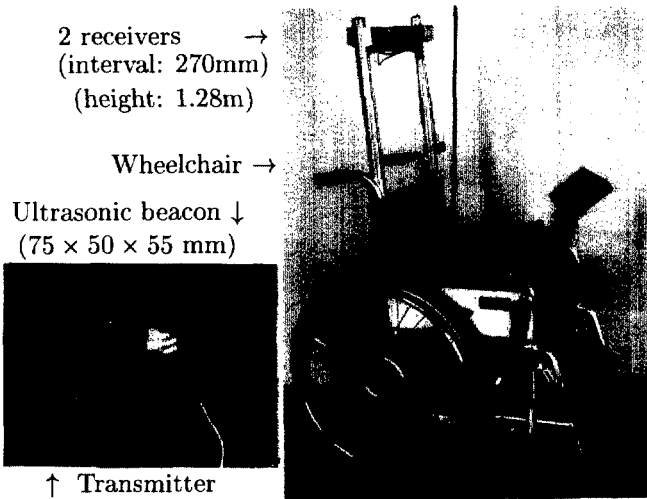
Figure 8: Developed beacons - wheelchair system
