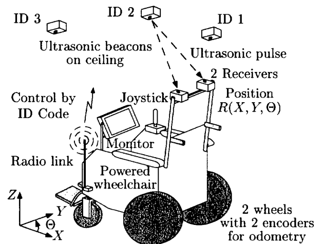
Figure 1: Navigation system using ultrasonic beacons
