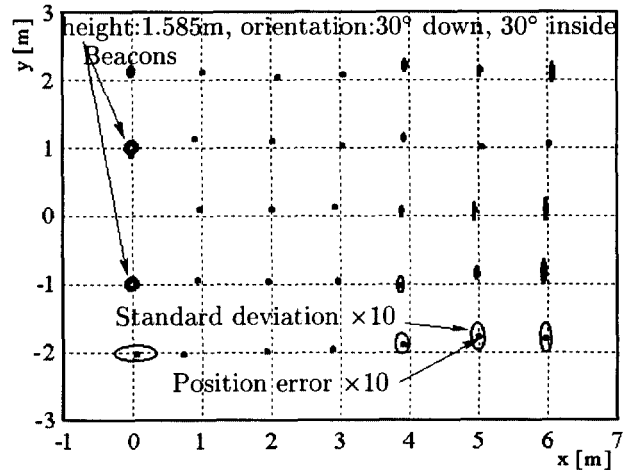
Positions at the cross points of 1m x 1m were measured. (Sampling: 10Hz 100times)
