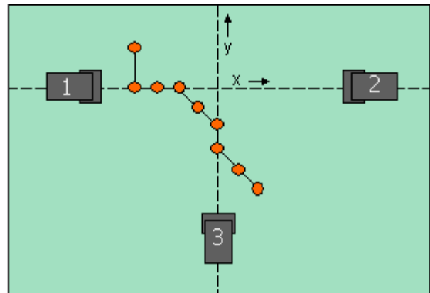
Figure 7. Experimental setup for validation. Ball locations marked as circles along trajectory. Dotted lines show the global coordinate frame.
