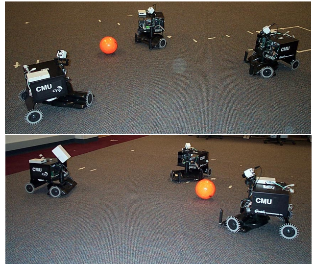
Figure 12. Blind robot ball tracking experiment setup. Top: In this experiment, three robots track the ball with a location generated by combining all three observations. Bottom: In this experiment, a robot is blinded (for example, a box covers the left robot's camera) and it still successfully tracks the ball with combined data from the remaining two.
