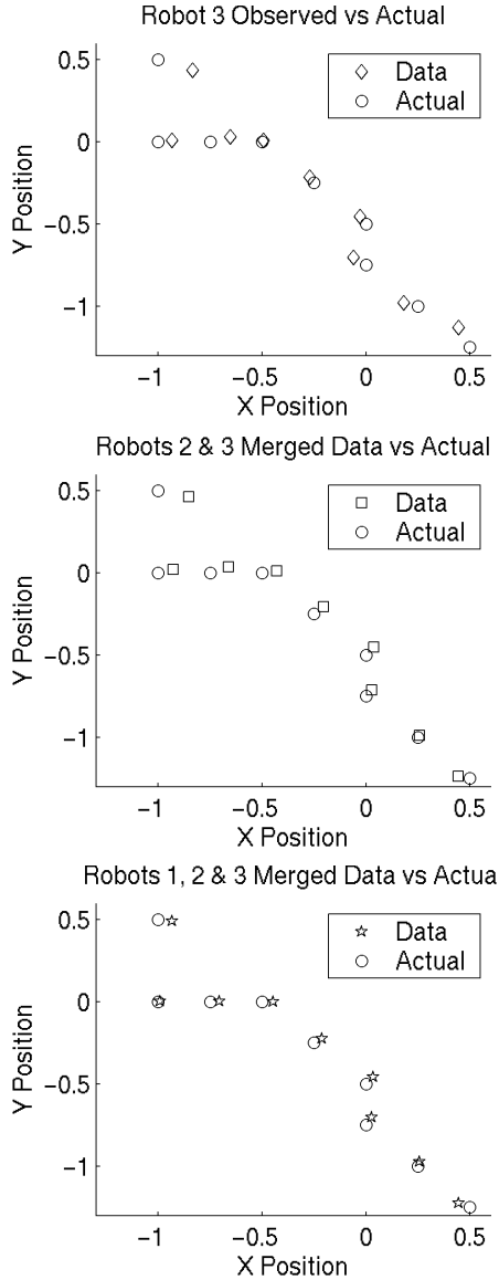
Figure 8. Reported data versus actual ball position. Top: Robot 3's estimate. Middle: Robots 2 and 3 merged estimates. Bottom: Robots 1, 2, and 3 merged estimates.
