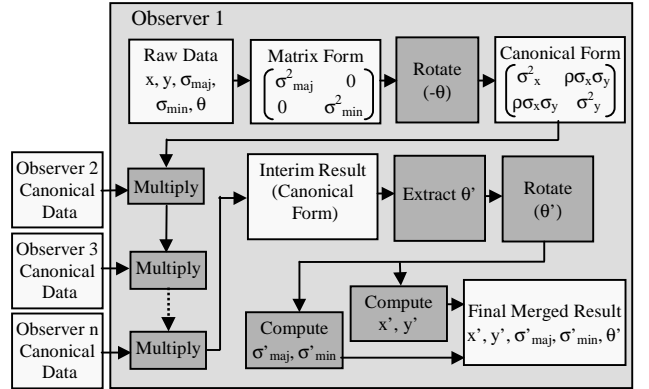
Figure 2. Block diagram representing the multi-distribution merging process. The multiplication step is conducted using the mathematical formulation described above. Each subsequent distribution is merged with the previous merging result.
