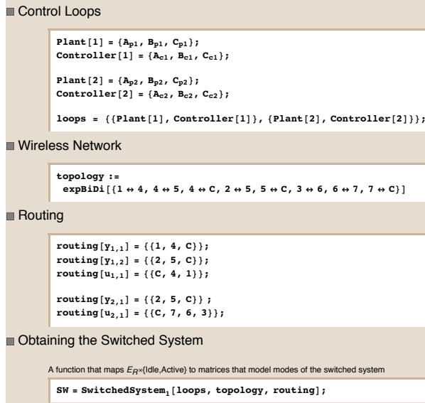
Fig. 9. A description of the multi-hop control network discussed in Section III and a computation of the corresponding switched system with the Mathematica based tool.
