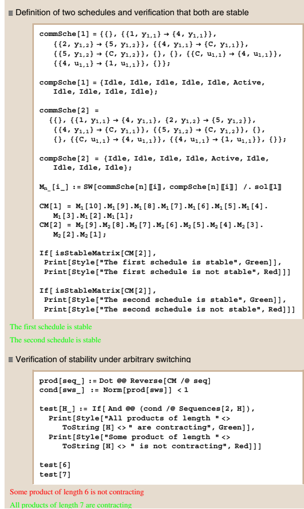
Fig. 11. Applying a sufficient condition for stability of switched systems to verify stability under non-deterministic network schedules.
