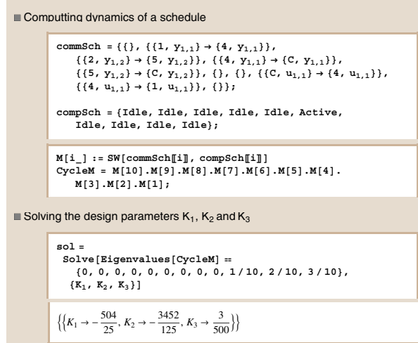
Fig. 10. Computation of matrix representing dynamics of a schedule and using it to assign values to design parameters.
