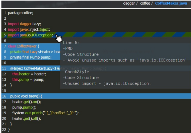
Fig. 4. Code-level view of UAV with Checkstyle and PMD warnings.
