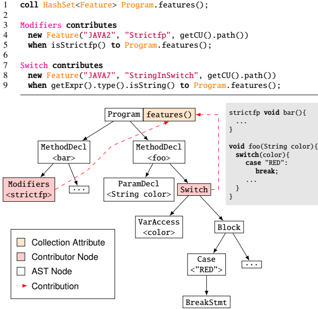
Fig. 1: Example definitions of features.
