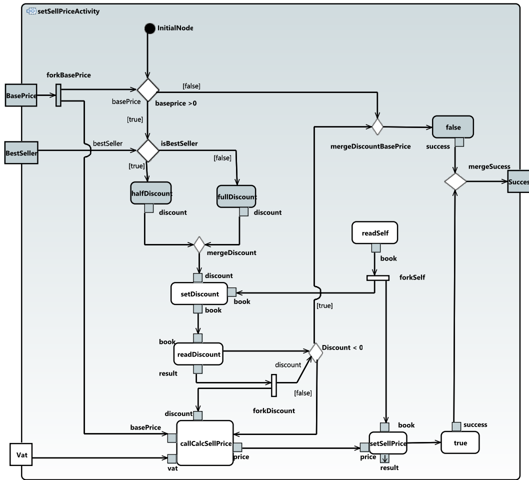
Fig. 3: fUML AD of setSellPriceActivity
