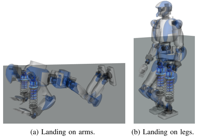
Fig. 1: Shock-absorber virtual-link dynamic model representation in two different landing configurations.
