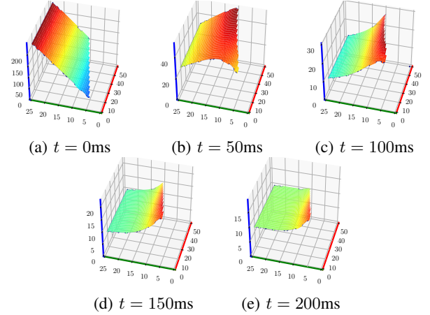
Fig. 6: Evolution of force f in N (blue axis), for a given stiffness K \in [0...50] in \text{N.m}^{-1} (red axis), and damping B \in [0...25] in \text{N.s.m}^{-1} (green axis).
