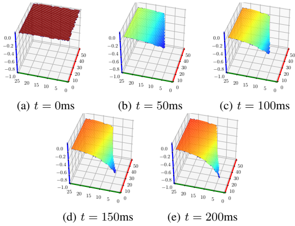
Fig. 4: Evolution of position z in m (blue axis), for a given stiffness K \in [0...50] in \text{N.m}^{-1} (red axis), and damping B \in [0...25] in \text{N.s.m}^{-1} (green axis).
