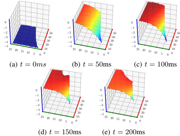
Fig. 5: Evolution of velocity \dot{z} in \text{m.s}^{-1} (blue axis), for a given stiffness K \in [0...50] in \text{N.m}^{-1} (red axis), and damping B \in [0...25] in \text{N.s.m}^{-1} (green axis).
