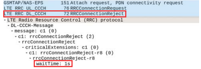
Fig. 7. Victim UE receives RRC Connection reject during BTS resource depletion attack .
