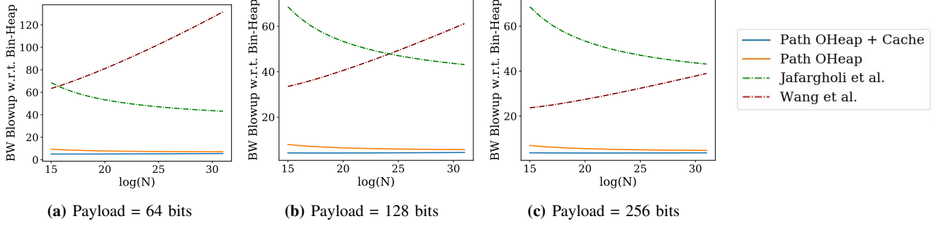
Fig. 1: Concrete Performance for Cloud Outsourcing. The orange curve represents Path Oblivious Heap where the client performs path-caching. The blue curves is when our Path Oblivious Heap performs path+treetop caching to match the client storage of Jafargholi et al. [25]. The green and the maroon curves represent prior works by Jafargholi et al. [25] and Wang et al. [44] respectively. In all figures, the comparison key is 32 bits and the per-request failure probability is at most 2^{-80} .
