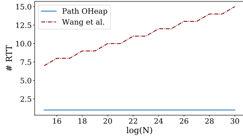
Fig. 2: Number of round trips. Wang et al. [44] incurs logarithmic roundtrips due to the recursion in the algorithm; in comparison, our algorithm incurs a single roundtrip per priority-queue request, assuming that the client can store O(1) tree-paths. Assuming small client storage, the worst-case number of round trips for Jafargholi et al. [25] is not in the visible region of the chart.
