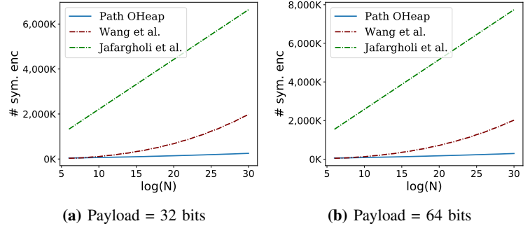
Fig. 3: Concrete Performance for MPC. The blue curve represents Path Oblivious Heap (the circuit-variant). The green and the maroon curves represent prior works by Jafargholi et al. [25] and Wang et al. [44] respectively. In all figures, the comparison key is 32 bits and the per-request failure probability is at most 2^{-80} .
