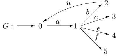
Fig. 1. Automaton of Example 2.
