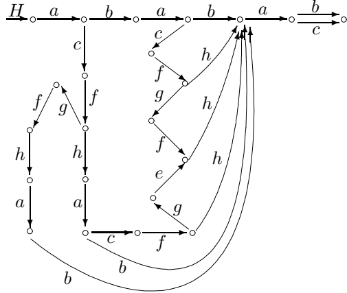
Fig. 3. Automaton H of Section V.
