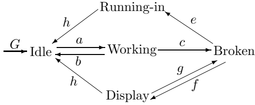
Fig. 2. Automaton G of Section V.
