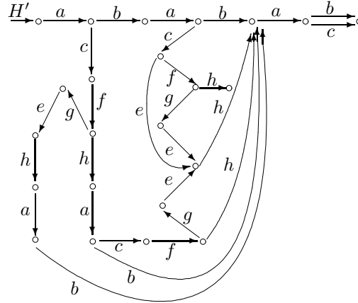
Fig. 4. Automaton H' of Section V.
