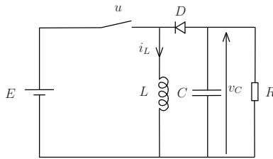
Figure 2: Buck-boost converter
