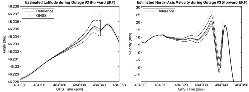
Fig. 9. Estimated Latitude (left panel) and North-axis velocity (right panel) using three subversions of the constructed model, together with the estimated 3- \sigma confidence levels.
