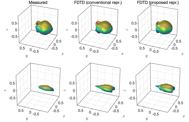
Fig. 4. Normalized balloon plots (in arbitrary units, a. u.) for the FDTD output of the data from Fig. 5 taken over a sphere of radius 0.75 m at a frequency of 818 Hz (top) and 5513 Hz (bottom). Left: measured directivity. Middle: 6th-order conventional representation. Right: 6th-order proposed representation.
