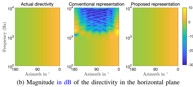
(b) Magnitude in dB of the directivity in the horizontal plane
