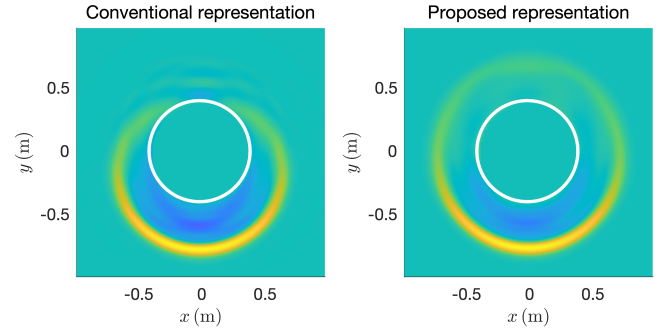
Fig. 5. Snapshot at t = 3.6 ms of a cross-section through the horizontal plane of the simulated acoustic field emitted by the IEM loudspeaker cube (cf. 4) using a Gaussian pulse of variance 1 \times 10^{-4} as input signal. Here, we use the directivity data of driver 1, with the conventional representation (left) and the proposed one (right), both of 6th order.
