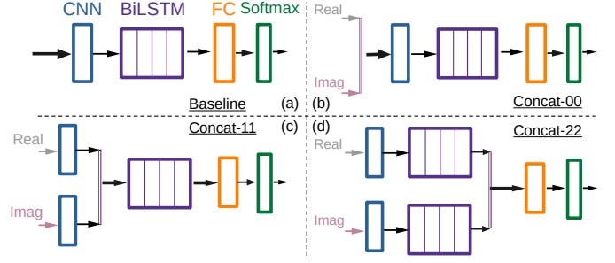
Fig. 7. Multi-stream acoustic models consisting of convolutional, recurrent (BiLSTM) and fully-connected (FC) layers. (a) Single-stream baseline, (b)-(d) multi-stream with fusion at different abstraction levels.
