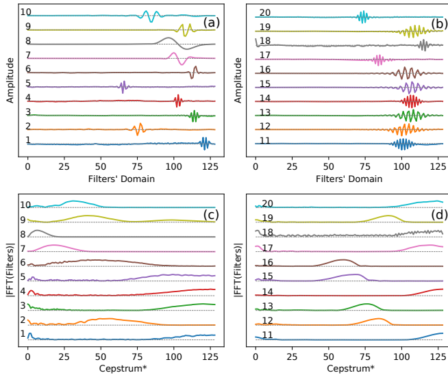
Fig. 19. The learned filters in the Conv-L1 which resemble (a) wavelets and (b) parametric functions (e.g., sinc), along with their |FFT| (c) and (d).
