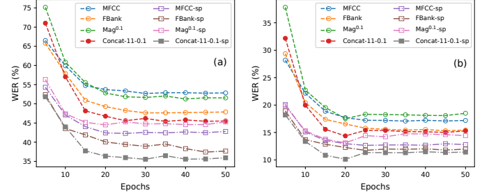
Fig. 16. WER vs epoch for TORGO (fold 1). (a) Dysarthric, (b) Typical.
