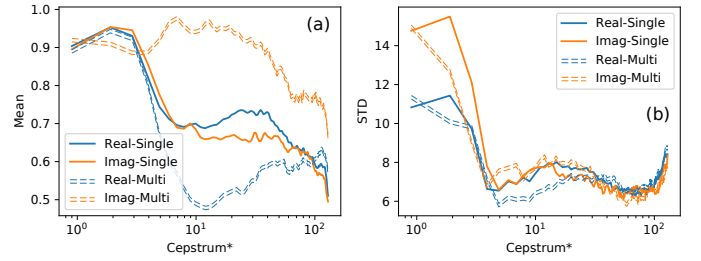
Fig. 18. Mean and STD of the Conv-L1's filters after taking |\text{FFT}| from the filters in the single-stream (Single) and multi-stream (Multi) systems (CNN+FC, WSJ) fed with the real and/or imaginary parts. (a) Mean, (b) STD.
