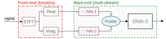
Fig. 5. The proposed multi-stream system fed with the real and imaginary parts of the FT. Each stream is pre-processed by (D)NN-1 and (D)NN-2 which can be (deep or) shallow. DNN-3 post-processes the fused streams.
