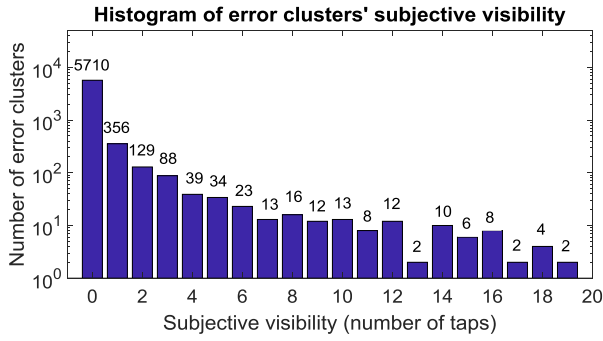
Fig. 7. Histogram for the error clusters classified by the number of detections (note the logarithmic scale for the Y-axis).
