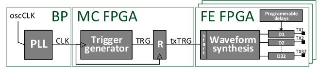
Fig. 1 TX signals generation. The txTRG signal, synchronous with CLK, initializes the generation of the 32 TX signals in each of the 8 FE boards. The actual delay of each signal start ( D_i ) can be arbitrarily programmed. The same CLK and txTRG signals are also used to synchronize all RX operations.
