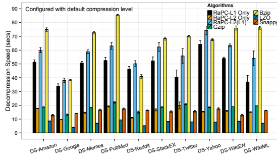
Fig. 8. RaPC decomposition speed comparing to Bzip , Gzip and LZO with default compression level .
