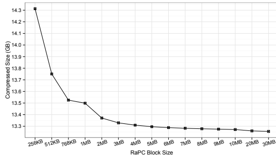
Fig. 4. RaPC Layer-2 block size verses compression ratios
