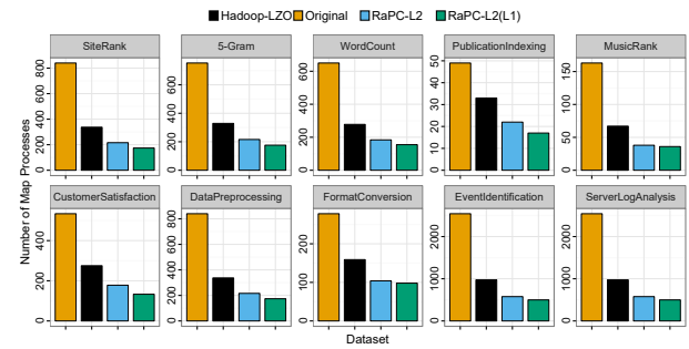
Fig. 5. Number of Map processes for each job (default to Hadoop) with original, RaPC-L2 compressed and RaPC-L2(L1) compressed data.
